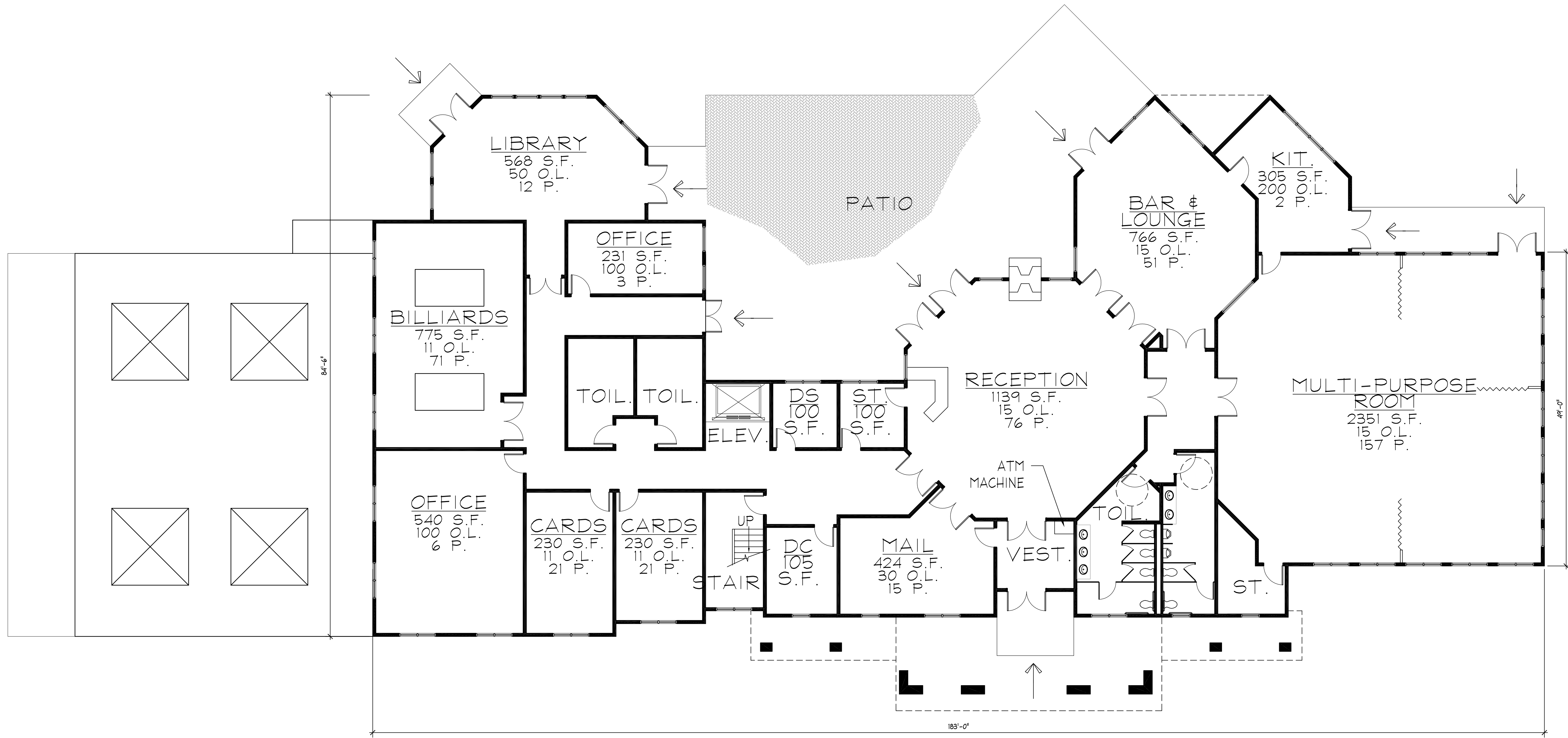
1 MAIN LEVEL FLOOR PLAN A1.31 1/8"=1'-0"
